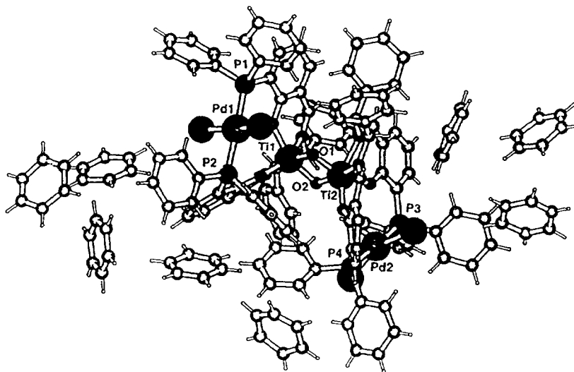
Figure 1. X-ray crystal structure of the complex 7. Selected bond lengths [Å] and angles [°]: Ti1-Ti2 2.812(3), Pd1-Ti1 4.177(8), Pd2-Ti2 4.134(7); Ti1-O1-Ti2 98.8(3), Ti1-O2-Ti2 96.6(3), P1-Pd-P2 177.8(1), P3-Pd-P4 176.8(1).
